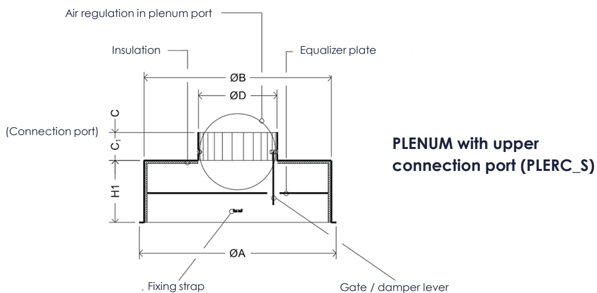
DIMENSION TABLE FOR PLENUM
